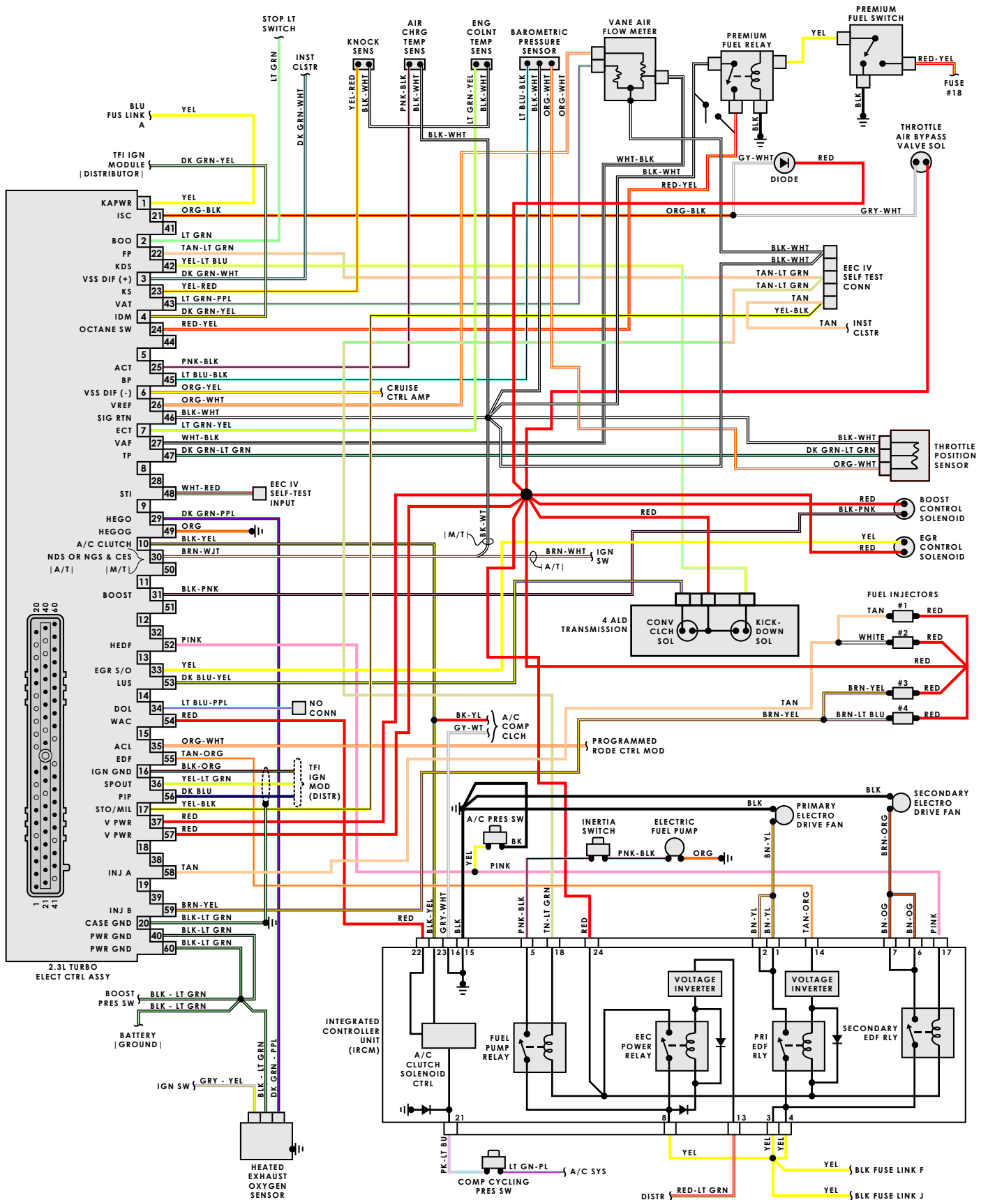
1988 Cougar/Thunderbird 2.3L Turbo Electronic Fuel Injection System Wiring Diagram
